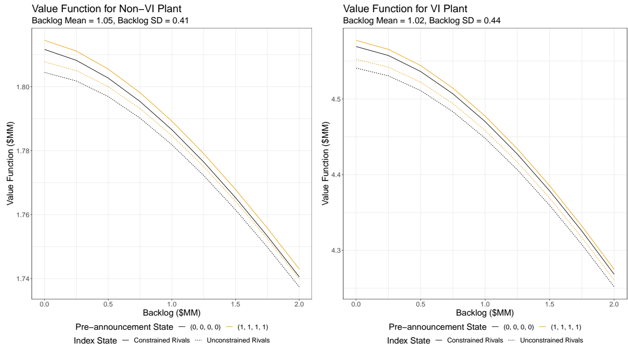
Figure 3: These figures show the value functions when near small, near large, medium small, and medium large auctions are available to bid on in period t (i.e. \mathbf{y}_{i,t} = 1 ). A pre-announcement state refers to \mathbf{x}_{i,t} as defined in the text. \mathbf{x}_{i,t} = 1 ( \mathbf{x}_{i,t} = 0 ) means the government issued pre-announcements which (did not) included auctions in the near small, near large, medium small, and medium large bins.
