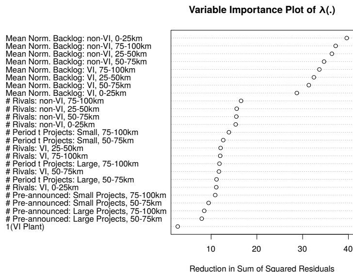
Figure 2: This plot shows the variable importance plot of the index function. Importance is measured as the total decrease in the sum of squared residuals from splitting on the variable. Values further to the right correspond to variables that are more important in the sense they helped the index fit the data better.
