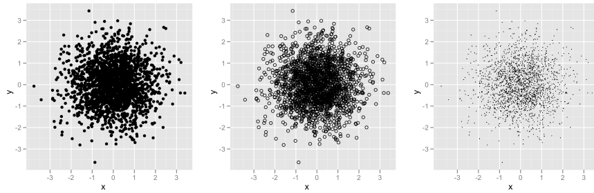
Fig. 5.7: Modifying the glyph used can help with mild to moderate overplotting. From left to right: the default shape, shape = 1 (hollow points), and shape = "." (pixel points).
