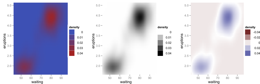
Fig. 6.7: Density of eruptions with three colour schemes. (Left) Default gradient colour scheme, (middle) customised gradient from white to black and (right) 3 point gradient with midpoint set to the mean density.
