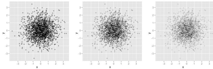
Fig. 5.8: Using alpha blending to alleviate overplotting in sample data from a bivariate normal. Alpha values from left to right: 1/3 , 1/5 , 1/10 .
