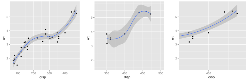
Fig. 7.13: Setting limits on the coordinate system, vs setting limits on the scales. (Left) Entire dataset; (middle) x scale limits set to (325, 500); (right) coordinate system x limits set to (325, 500). Scaling the coordinate limits performs a visual zoom, while setting the scale limits subsets the data and refits the smooth.
