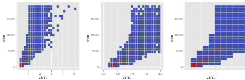
Fig. 7.14: Setting limits on the coordinate system, vs. setting limits on the scales. (Left) Entire dataset; (middle) x scale limits set to (0, 2); (right) coordinate x limits set to (0, 2). Compare the size of the bins: when you set the scale limits, there are the same number of bins but they each cover a smaller region of the data; when you set the coordinate limits, there are fewer bins and they cover the same amount of data as the original.
