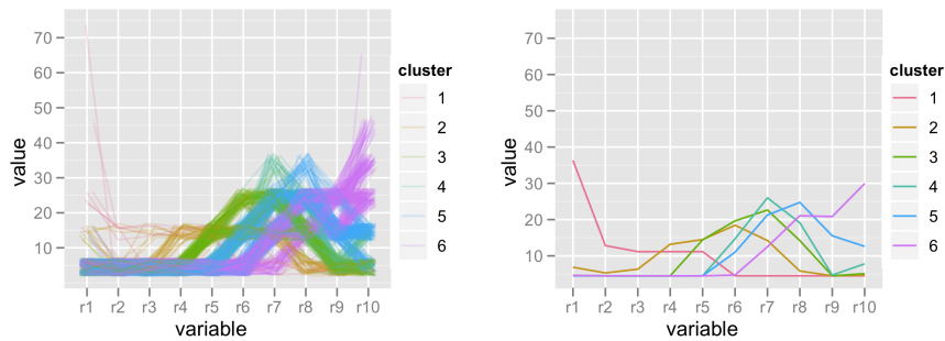
Fig. 9.7: Displaying cluster membership on a parallel coordinates plot. (Left) Individual movies coloured by group membership and (right) group means.
