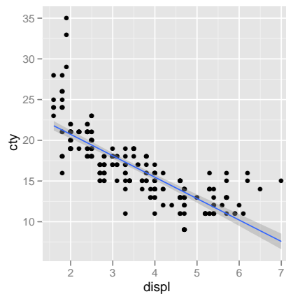
Fig. 9.10: A simple linear model that doesn't fit the data very well.
