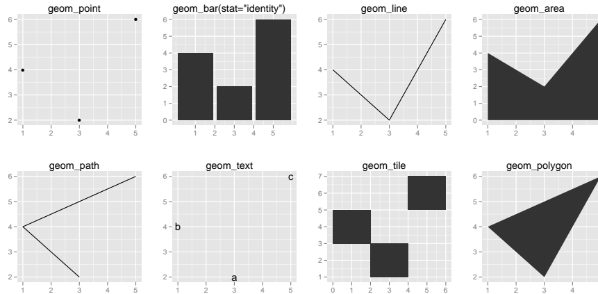
Fig. 5.1: The basic geoms applied to the same data. Many give rise to named plots (from top left to bottom right): scatterplot, bar chart, line chart, area chart, path plot, labelled scatterplot, image/level plot and polygon plot. Observe the different axis ranges for the bar, area and tile plots: these geoms take up space outside the range of the data, and so push the axes out.
