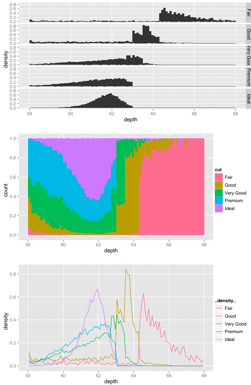
Fig. 5.3: Three views of the distribution of depth and cut. From top to bottom: faceted histogram, a conditional density plot, and frequency polygons. All show an interesting pattern: as quality increases, the distribution shifts to the left and becomes more symmetric.
