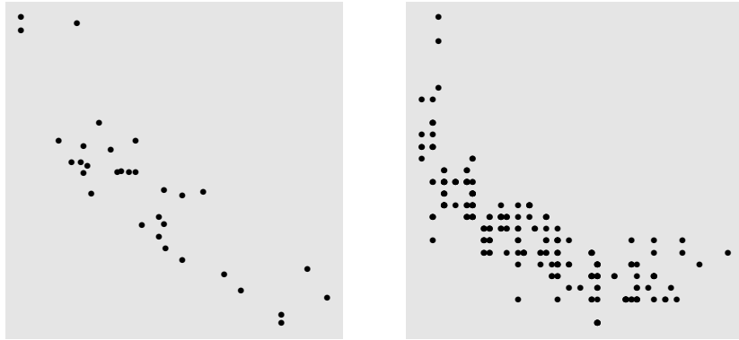
Fig. 10.3: Using “quiet” x and y scales removes the labels and hides ticks and gridlines.
