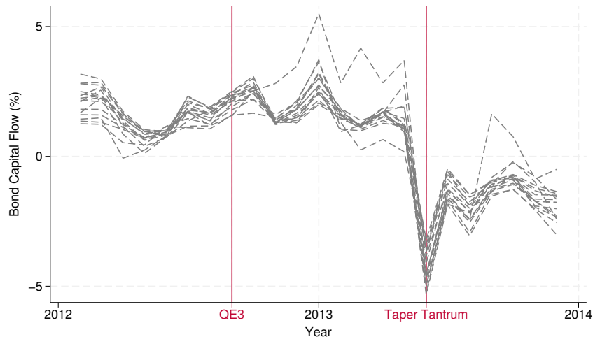
Figure 1: Quantitative Tightening in the U.S. and Capital Flows to Emerging Markets
