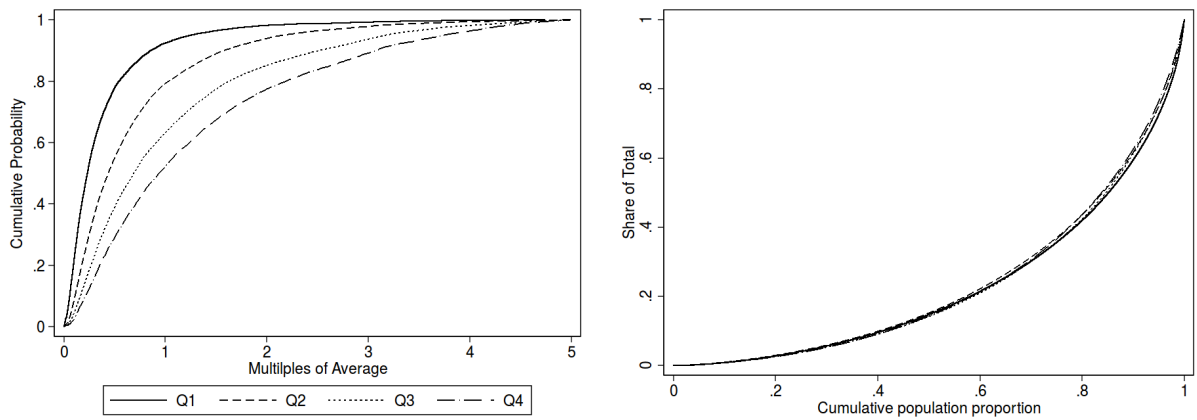
(b) Case 2: conditional distributions of z_h by a_{-1} quartiles
