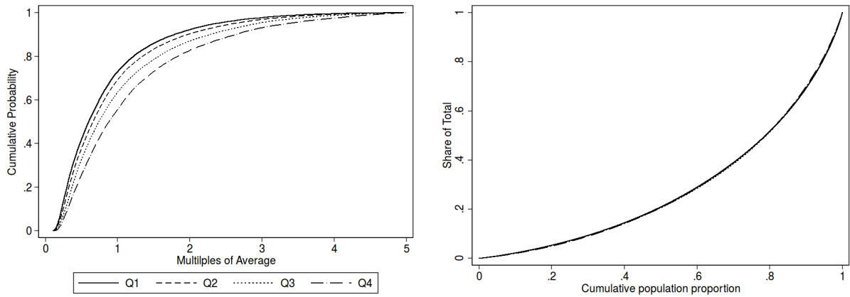
(a) Case 4: conditional distributions of c_v by a_{-1} quartiles
