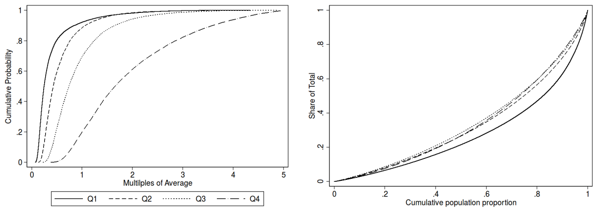
(c) Case 3: conditional distributions of z_w by z_{h,-1} quartiles
