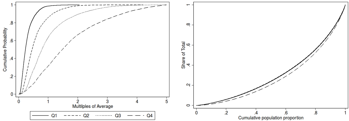
(a) Case 1: conditional distributions of z_h by z_{h,-1} quartiles
