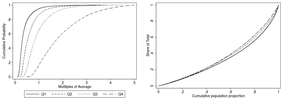
(b) Case 5: conditional distributions of c_v by z_{h,-1} quartiles
